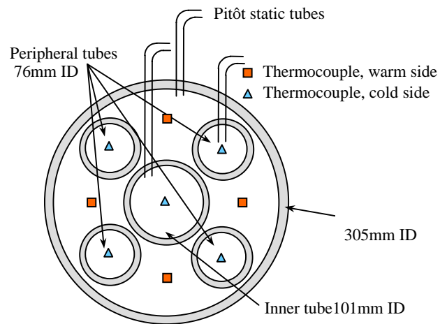
Figure 1: Schematic of the prototype cross-section
