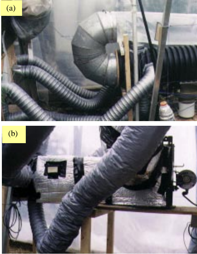
Figure 2: (a) Warm end of the unit; (b) Cold end of the unit
