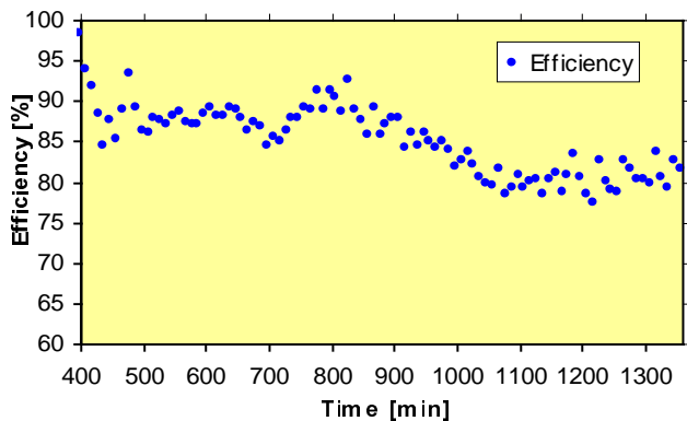
Figure 5: Variation of efficiency with time. March 26th, 1996: 0.5 air chg / h
