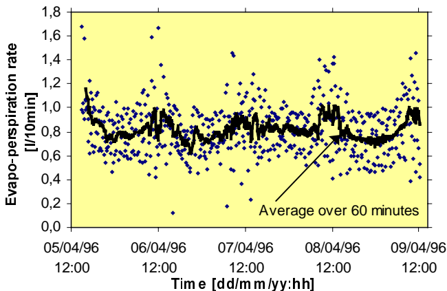
Figure 8: Rate of transpiration (not condensed on the walls) between April 5 th and 9 th 1996
