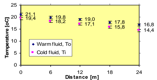
Figure 4: Temperature distribution. April 30th, 1996: 18h10, 0.9 air chg / h
