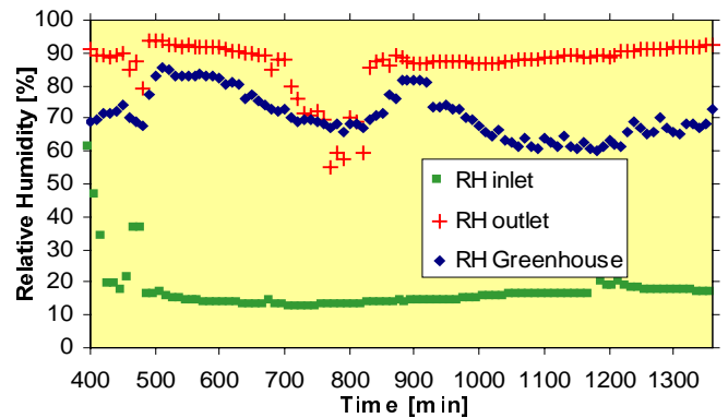
Figure 6: Relative humidity distribution in the greenhouse on March 26th 1996: 0.5 air chg / h.
