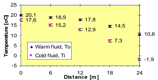
Figure 3: Temperature distribution. March 26th, 1996: 8h10, 0.5 air chg / h
